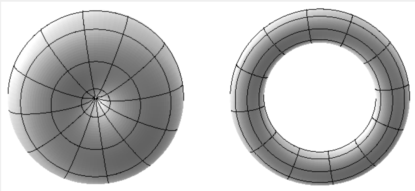
Figure 9-5 : Texture-Map Distortion
