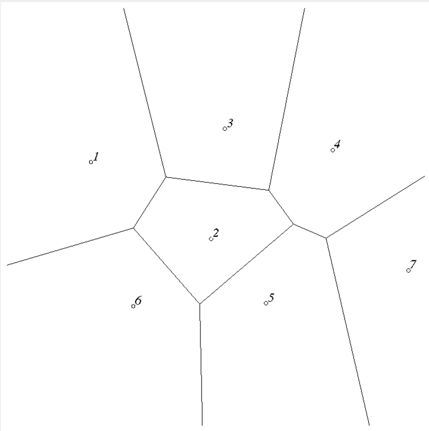
Figure 13-3 : Dirichlet Domains
