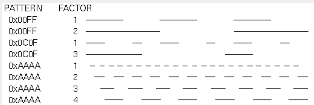
Figure 2-7 : Stippled Lines
