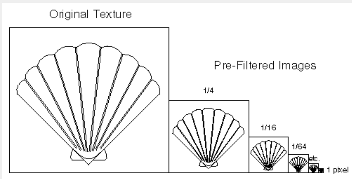
Figure 9-3 : Mipmaps
