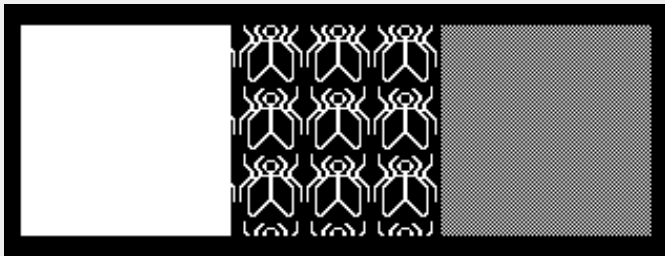
Figure 2-10 : Stippled Polygons
