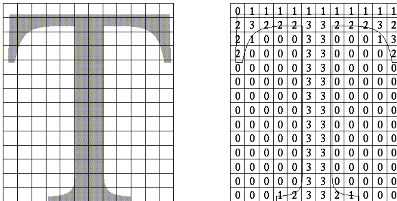
Figure 13-1 : Antialiased Characters
