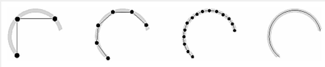
Figure 2-4 : Approximating Curves
