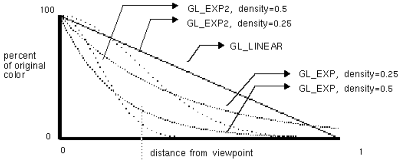
Figure 7-4 : Fog-Density Equations
