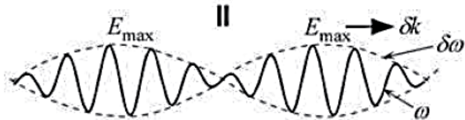
A periodic wave packet
