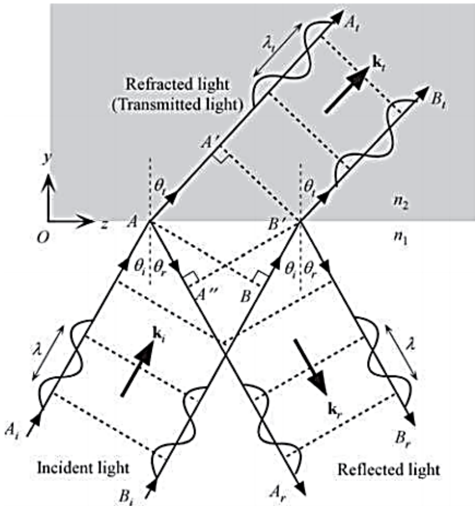
FIGURE 1.11 A light wave traveling in a medium with a greater refractive index ( n_1 > n_2 ) suffers reflection and refraction at the boundary. (Notice that \lambda_t is slightly longer than \lambda .)
