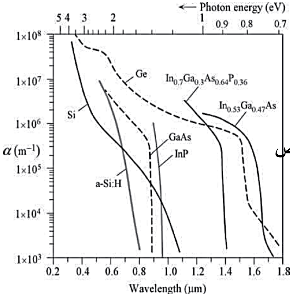
Absorption coefficient ( \alpha ) vs. wavelength ( \lambda ) for various semiconductors. (Data selectively collected and combined from various sources.)
