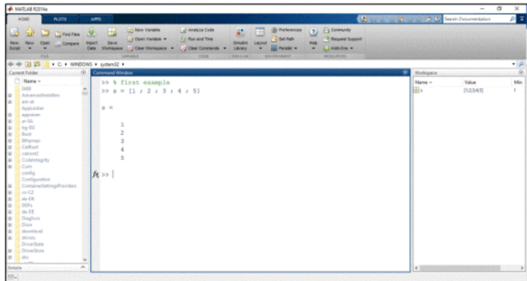
Fig 1.5. Define a column vector
