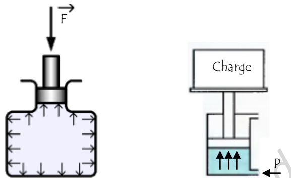
Figure 2 : Principe de Pascal (transmission de pression)
